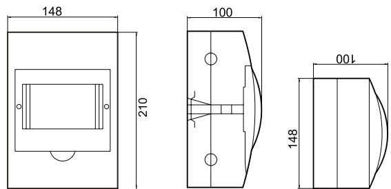
JHSA06 明盒 06 回路 Surface Mounted MCB Enclosure 06ways
