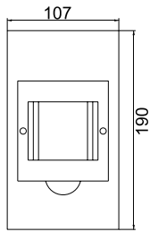
暗盒 4 回路 Flush Mounted MCB Enclosure 4ways
