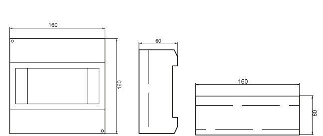
JHSH08 明盒 8 回路 Surface Mounted MCB Box 8ways
