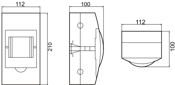
JHSA04 明盒 04 回路 Surface Mounted MCB Enclosure 04ways
