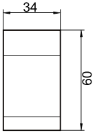
明盒 1 回路 Surface Mounted MCB Box 1way
