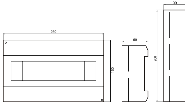
JHSH12 明盒 12 回路 Surface Mounted MCB Box 12ways
