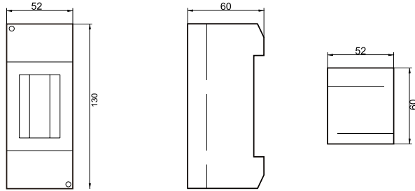
JHSH01 明盒 2 回路 Surface Mounted MCB Box 2ways
