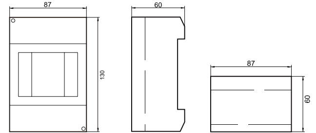
JHSH04 明盒 4 回路 Surface Mounted MCB Box 4ways
