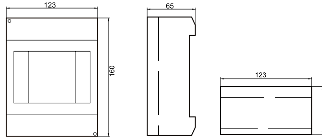
JHSH06 明盒 6 回路 Surface Mounted MCB Box 6ways
